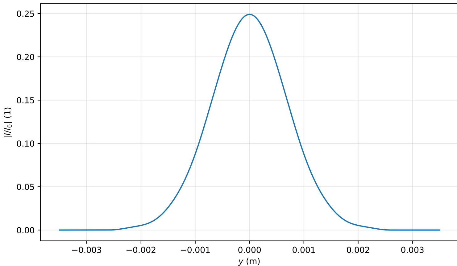
Intensity profile I(x=0, y, z=3.981)/I_0 , P_{in}=0.2P_{cr} , artificial time
